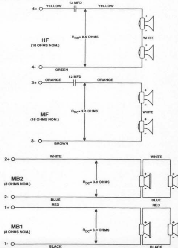
FIGURE 7 — Wiring Diagram
