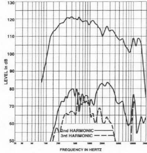
FIGURE 6 — Harmonic Distortion
