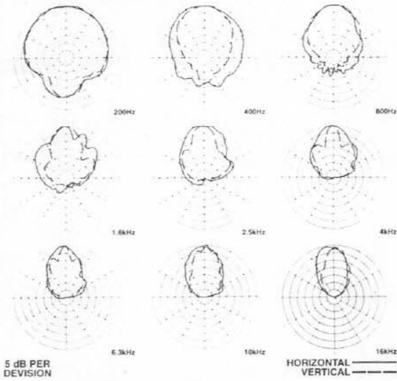
FIGURE 3 — Polar Response
